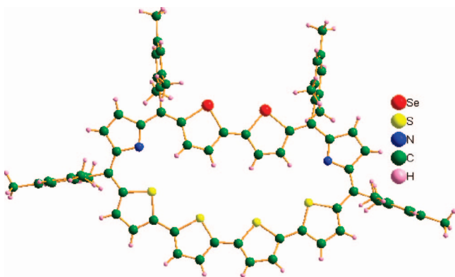
FIGURE 9. X-ray structure of 60a .
